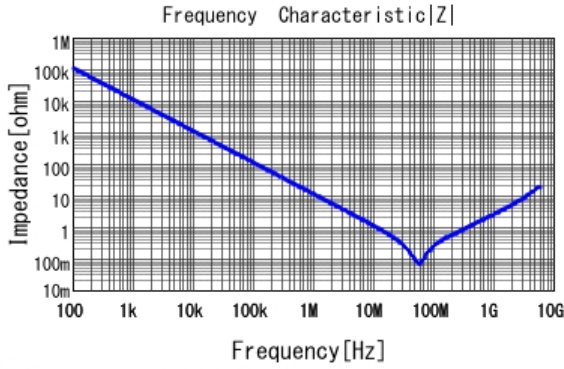
■ GRM188R71H153JA01 |Z| DCOV, 25degC
