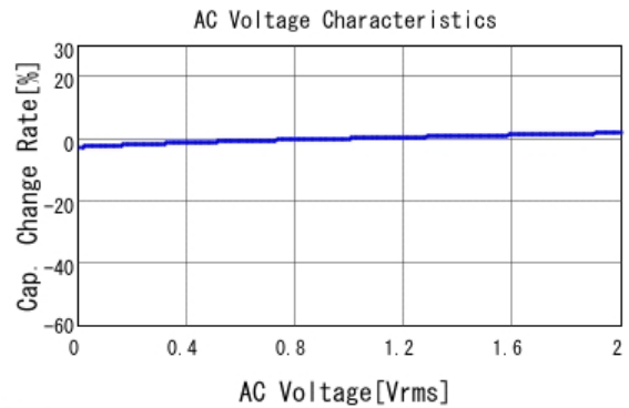
■ GRM188R71H153JA01 C-AC Voltage capchange, DCOV, 25.0d
