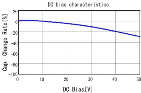
■ GRM188R71H153JA01 C-DC bias capchange, 25.0degC, AC1.
