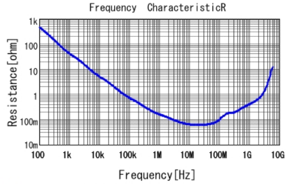
■ GRM188R71H153JA01 R DCOV, 25degC
