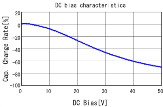
■ GRM188R71H154KAC4 C-DC bias capchange, 25.0degC, AC1.
