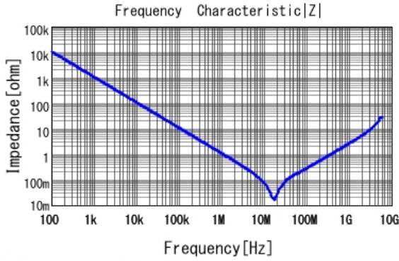
■ GRM188R71H154KAC4 |Z| DCOV, 25degC
