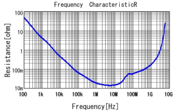
■ GRM188R71H154KAC4 R DCOV, 25degC
