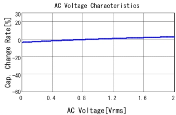
■ GRM188R71H154KAC4 C-AC Voltage capchange, DCOV, 25.0d
