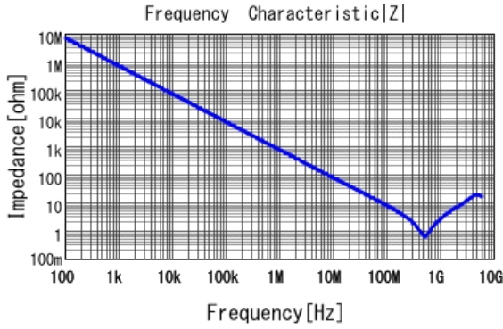
■ GRM188R71H221MA01 |Z| DCOV, 25degC
