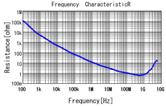
■ GRM188R71H221MA01 R DCOV, 25degC
