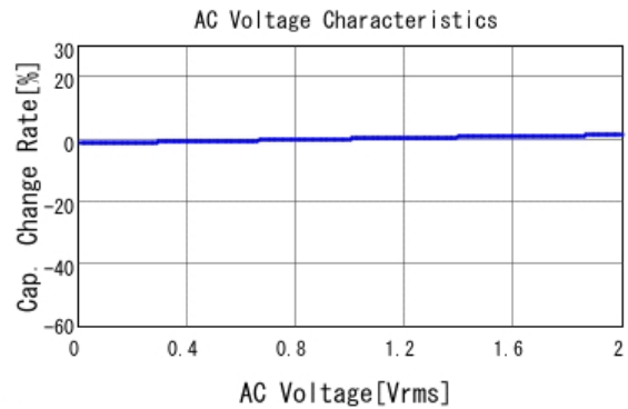
■ GRM188R71H221MA01 C-AC Voltage capchange, DCOV, 25.0d
