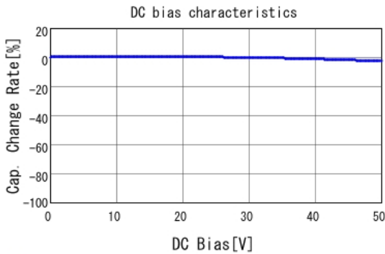
■ GRM188R71H221MA01 C-DC bias capchange, 25.0degC, AC1.
