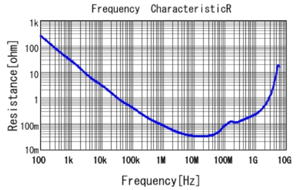
■ GRM188R71H273KA61 R DCOV, 25degC
