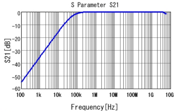
■ GRM188R71H273KA61 S21 DC0V, 25degC
