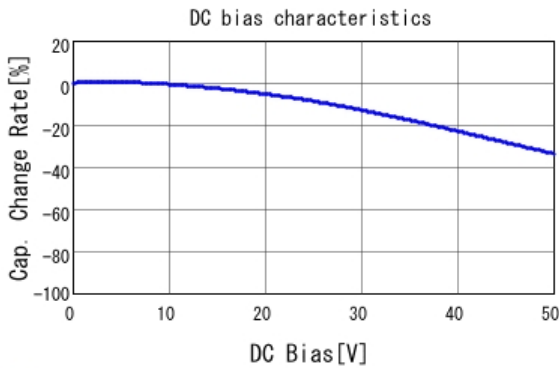
■ GRM188R71H273KA61 C-DC bias capchange, 25.0degC, AC1.
