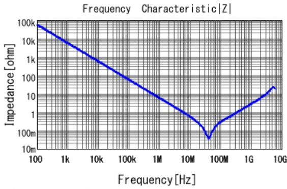
■ GRM188R71H273KA61 |Z| DCOV, 25degC
