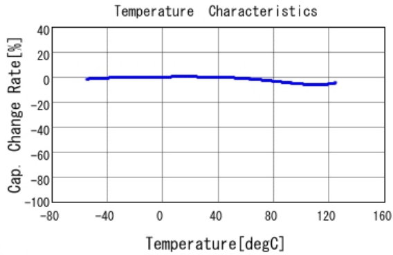
■ GRM188R71H273KA61 C-Temp. capchange, DC0.0V, AC1.0V rm
