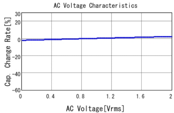
■ GRM188R71H273KA61 C-AC Voltage capchange, DCOV, 25.0d
