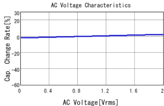
■ GRM188R71H333KA61 C-AC Voltage capchange, DCOV, 25.0d
