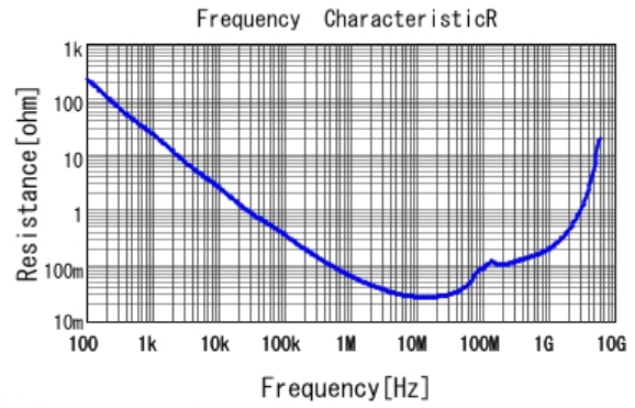
■ GRM188R71H333KA61 R DCOV, 25degC
