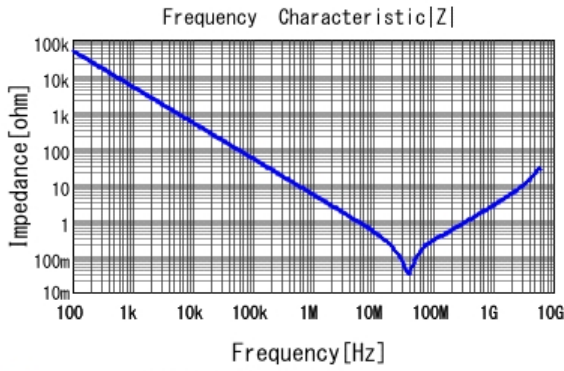
■ GRM188R71H333KA61 |Z| DCOV, 25degC
