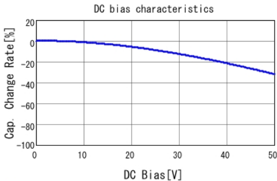
■ GRM188R71H333KA61 C-DC bias capchange, 25.0degC, AC1.
