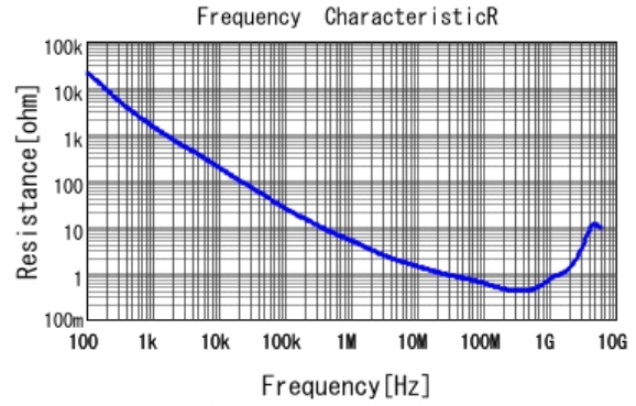
■ GRM188R71H471KA01 R DCOV, 25degC
