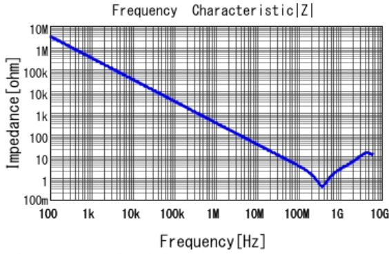
■ GRM188R71H471KA01 |Z| DCOV, 25degC
