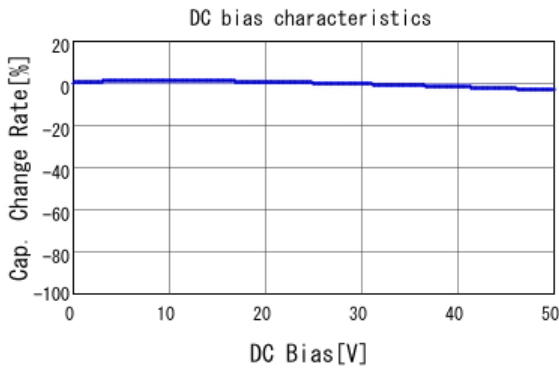
■ GRM188R71H471KA01 C-DC bias capchange, 25.0degC, AC1.
