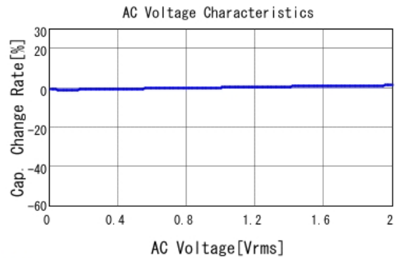
■ GRM188R71H471KA01 C-AC Voltage capchange, DCOV, 25.0d
