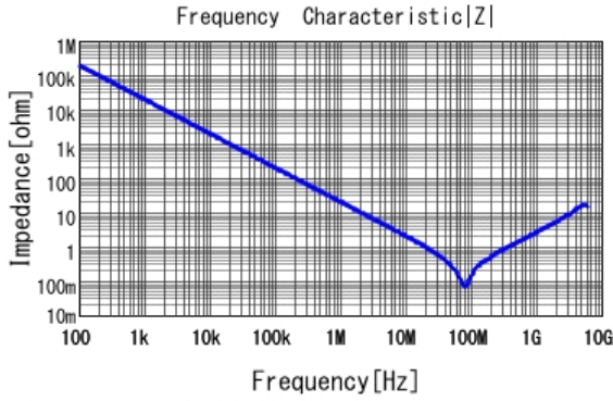
■ GRM188R71H822KA01 |Z| DCOV, 25degC
