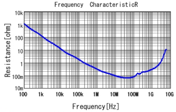
■ GRM188R71H822KA01 R DCOV, 25degC
