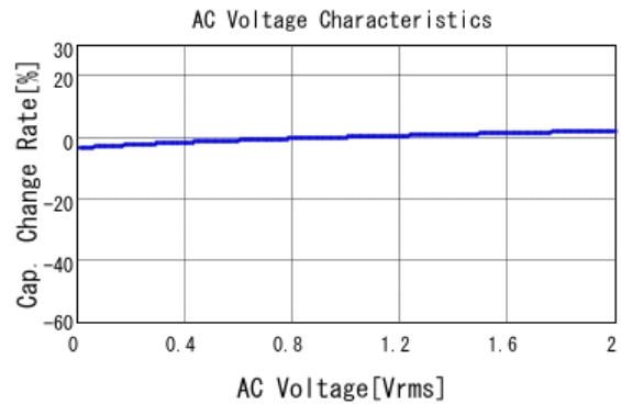
■ GRM188R71H822KA01 C-AC Voltage capchange, DCOV, 25.0d
