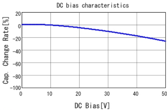
■ GRM188R71H822KA01 C-DC bias capchange, 25.0degC, AC1.
