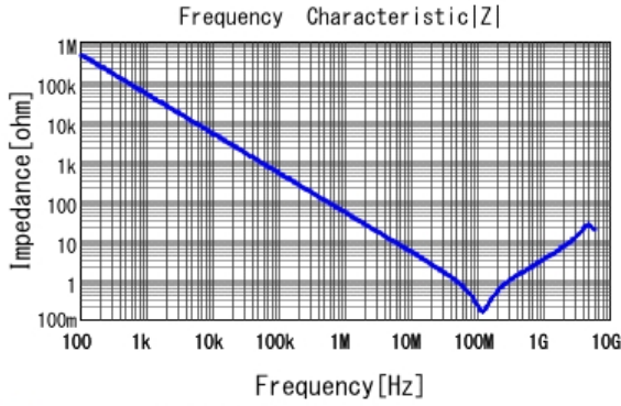
■ GRM188R72A332KA01 |Z| DCOV, 25degC
