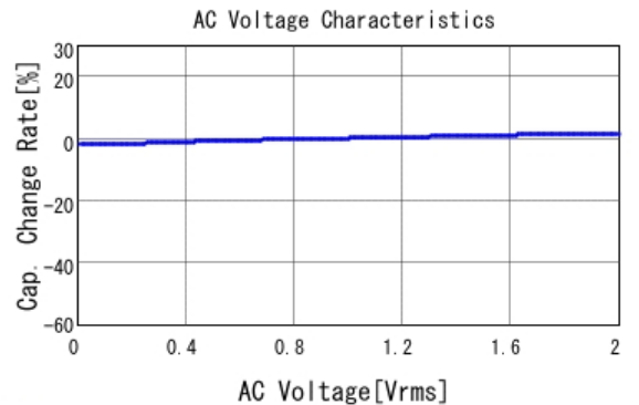
■ GRM188R72A332KA01 C-AC Voltage capchange, DCOV, 25.0d
