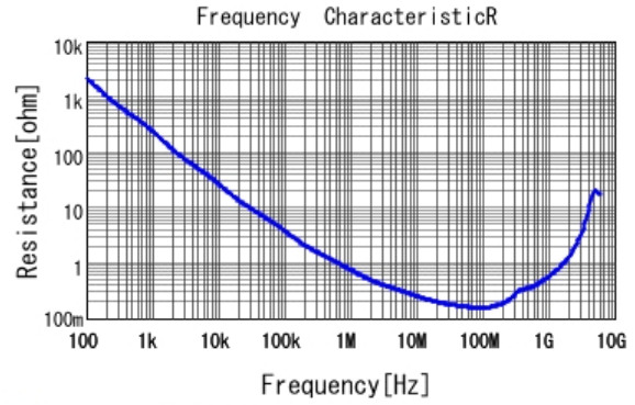
■ GRM188R72A332KA01 R DCOV, 25degC
