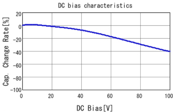
■ GRM188R72A332KA01 C-DC bias capchange, 25.0degC, AC1.
