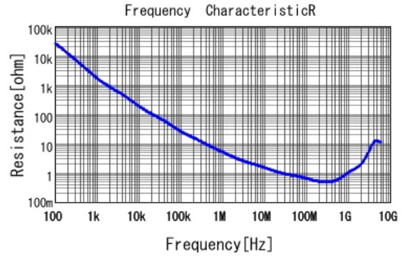
■ GRM188R72A471KA01 R DCOV, 25degC
