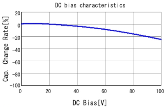
■ GRM188R72A471KA01 C-DC bias capchange, 25.0degC, AC1.
