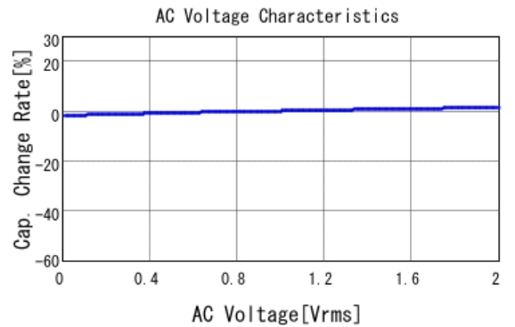
■ GRM188R72A471KA01 C-AC Voltage capchange, DCOV, 25.0d
