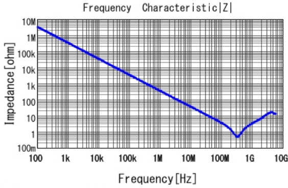
■ GRM188R72A471KA01 |Z| DCOV, 25degC
