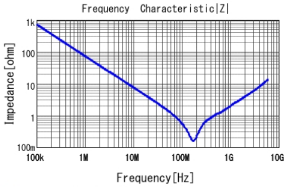
■ GRM188R72E222KW07 |Z| DCOV, 25degC
