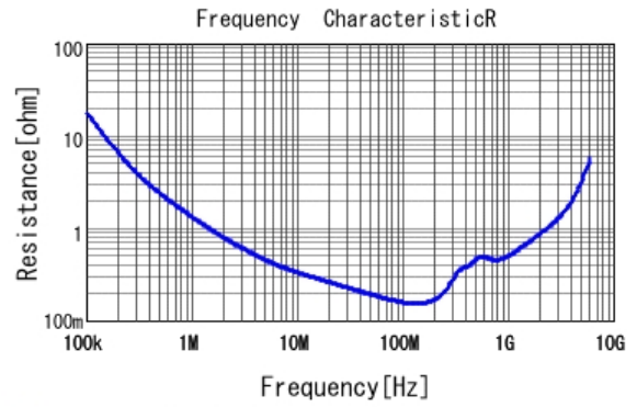
■ GRM188R72E222KW07 R DCOV, 25degC
