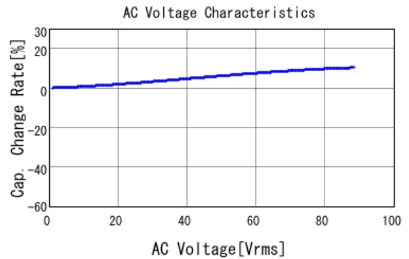
■ GRM188R72E222KW07 C-AC Voltage capchange, DCOV, 25.0d
