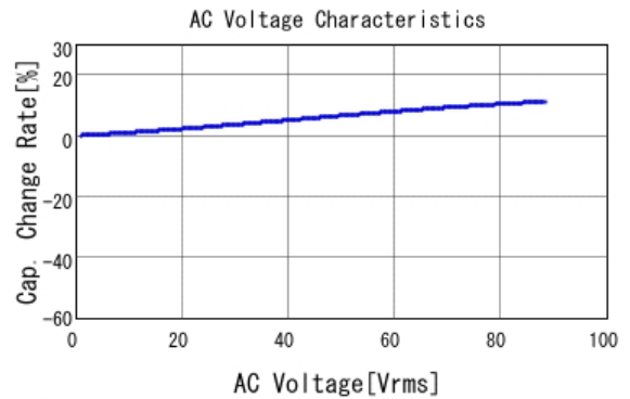
■ GRM188R72E331KW07 C-AC Voltage capchange, DCOV, 25.0d
