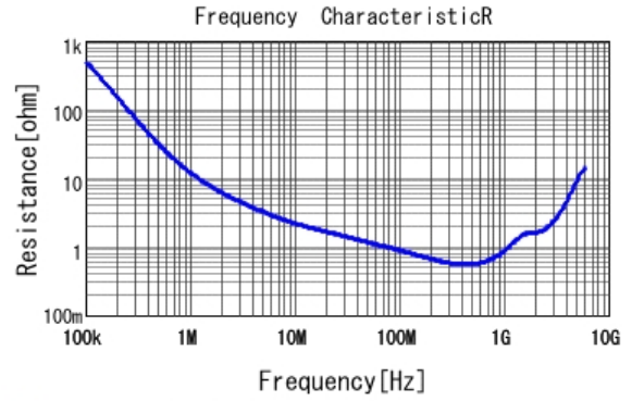
■ GRM188R72E331KW07 R DCOV, 25degC
