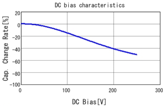
■ GRM188R72E331KW07 C-DC bias capchange, 25.0degC, AC1V
