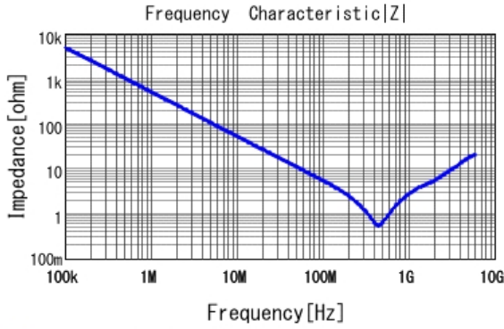
■ GRM188R72E331KW07 |Z| DCOV, 25degC
