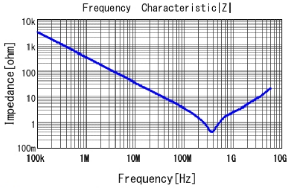
■ GRM188R72E471KW07 |Z| DCOV, 25degC
