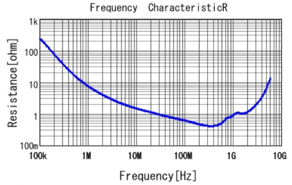
■ GRM188R72E471KW07 R DCOV, 25degC
