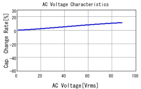
■ GRM188R72E471KW07 C-AC Voltage capchange, DCOV, 25.0d
