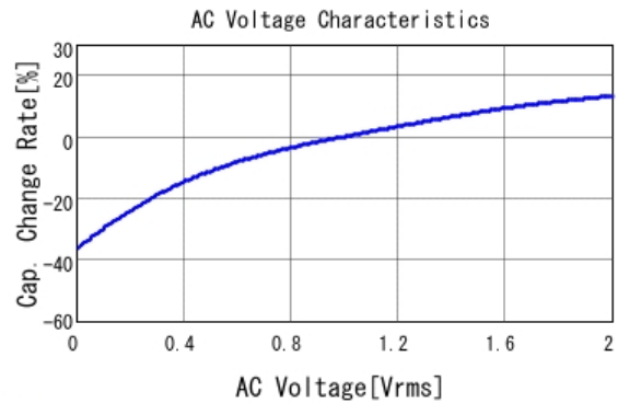
■ GRM188R7YA105KA12 C-AC Voltage capchange, DCOV, 25.0d
