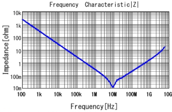
■ GRM188R7YA105KA12 |Z| DCOV, 25degC
