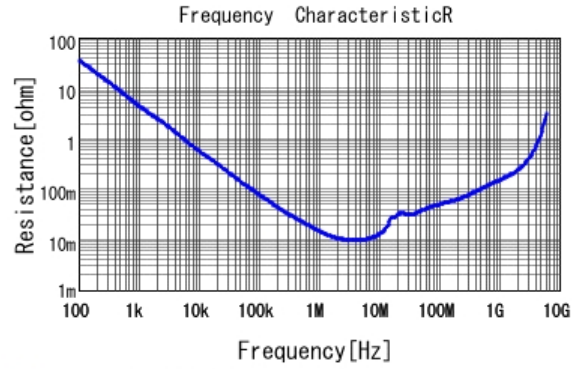
■ GRM188R7YA105KA12 R DCOV, 25degC
