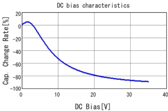
■ GRM188R7YA105KA12 C-DC bias capchange, 25.0degC, AC1.
