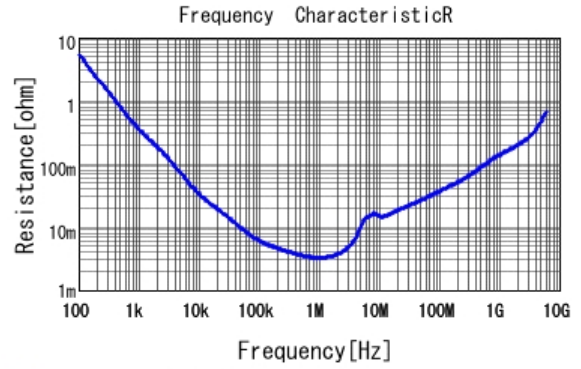
■ GRM188Z71C475KE21 R DCOV, 25degC
