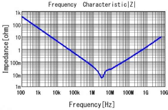
■ GRM188Z71C475KE21 |Z| DCOV, 25degC
