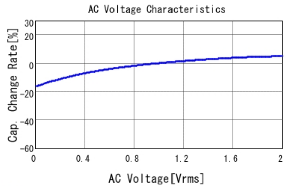
■ GRM188Z71C475KE21 C-AC Voltage capchange, DCOV, 25.0d
