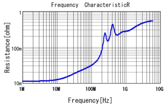
■ GRM2162C1H472JA01 R DCOV, 20degC
