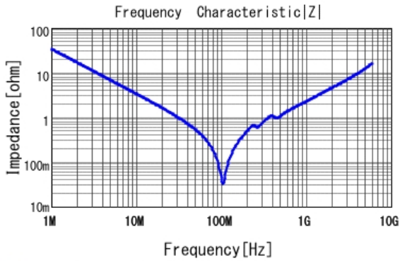
■ GRM2162C1H472JA01 |Z| DCOV, 20degC
