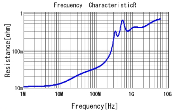
■ GRM2165C1H222JA01 R DCOV, 25degC
