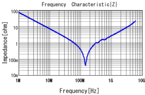
■ GRM2165C1H222JA01 |Z| DCOV, 25degC
