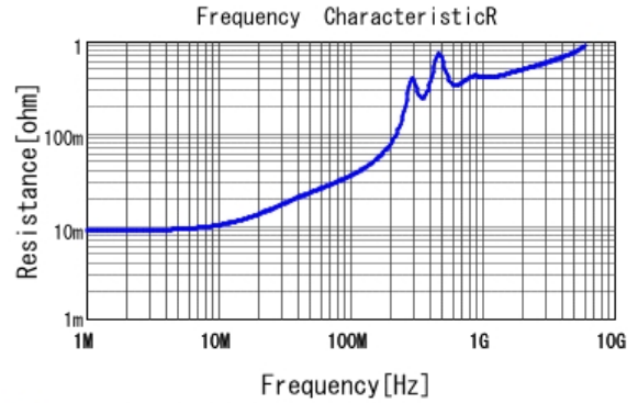
■ GRM2165C1H272JA01 R DCOV, 25degC
