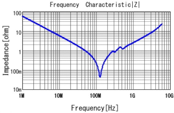
■ GRM2165C1H272JA01 |Z| DCOV, 25degC
