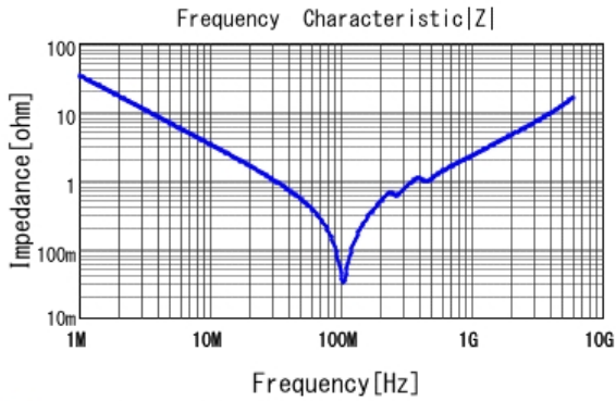
■ GRM2165C1H472JA01 |Z| DCOV, 25degC
