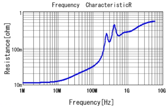
■ GRM2165C1H472JA01 R DCOV, 25degC
