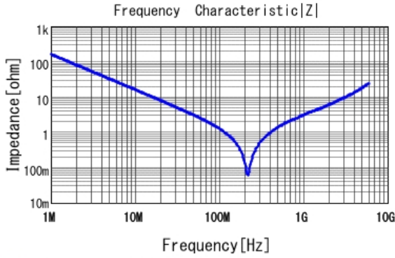
■ GRM2165C2A102JA01 |Z| DCOV, 25degC
