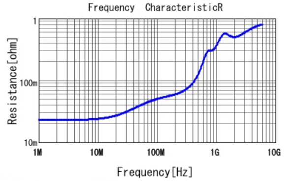
■ GRM2165C2A102JA01 R DCOV, 25degC
