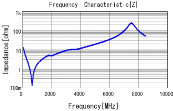
■ GRM2165C2A121JA01 |Z| DCOV, 25degC
