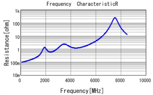
■ GRM2165C2A121JA01 R DCOV, 25degC
