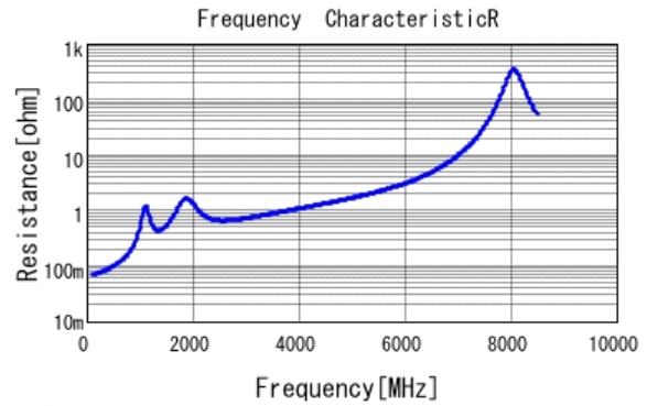
■ GRM2165C2A271JA01 R DCOV, 25degC
