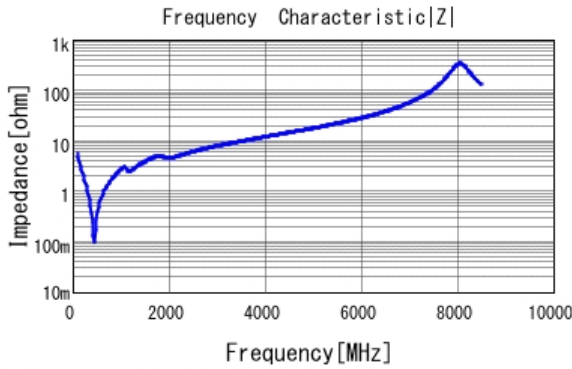
■ GRM2165C2A271JA01 |Z| DCOV, 25degC
