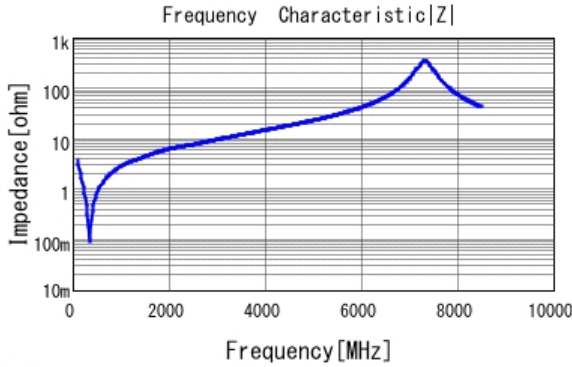
■ GRM2165C2A391JA01 |Z| DCOV, 25degC
