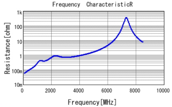
■ GRM2165C2A391JA01 R DCOV, 25degC
