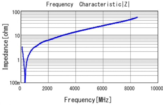
■ GRM2165C2A471JA01 |Z| DCOV, 25degC
