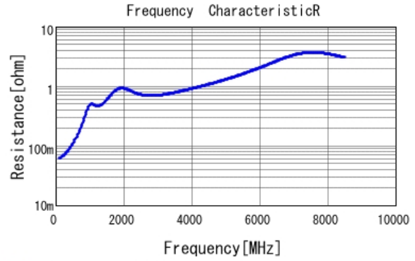
■ GRM2165C2A471JA01 R DCOV, 25degC
