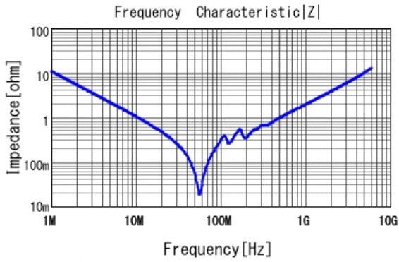
■ GRM2195C1H153JA01 |Z| DCOV, 25degC
