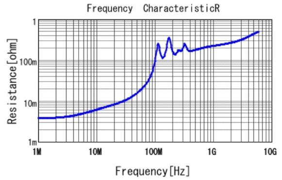
■ GRM2195C1H153JA01 R DCOV, 25degC
