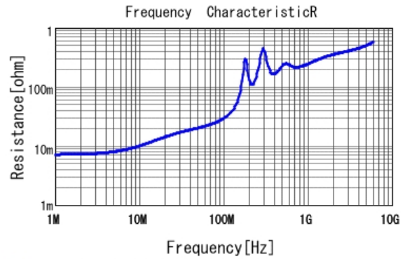
■ GRM2195C1H682JA01 R DCOV, 25degC
