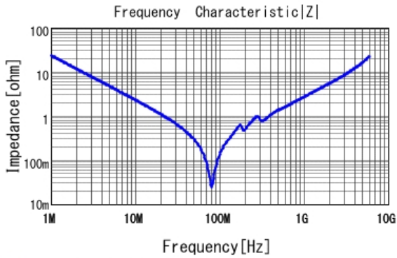
■ GRM2195C1H682JA01 |Z| DCOV, 25degC
