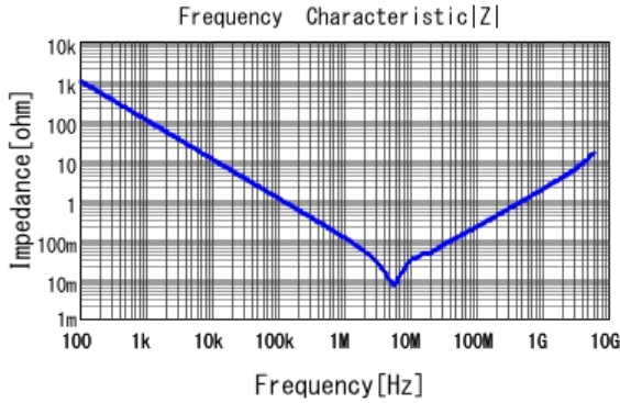
■ GRM219B31H225KE15 |Z| DCOV, 20degC
