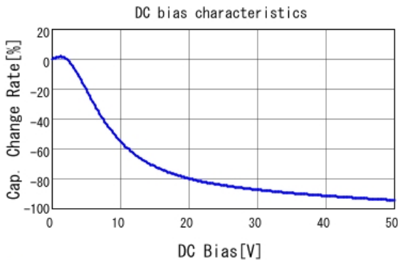
■ GRM219B31H225KE15 C-DC bias capchange, 20.0degC, AC1.
