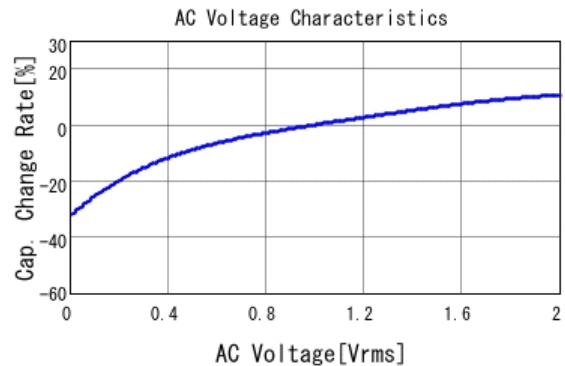
■ GRM219B31H225KE15 C-AC Voltage capchange, DCOV, 20.0d
