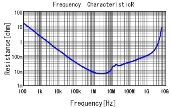
■ GRM219B31H225KE15 R DCOV, 20degC
