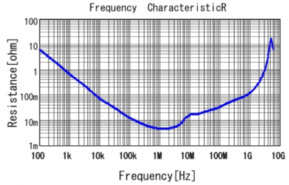
■ GRM219C71C475ME21 R DCOV, 25degC
