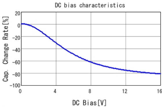
■ GRM219C71C475ME21 C-DC bias capchange, 25.0degC, AC1V
