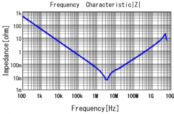
■ GRM219C71C475ME21 |Z| DCOV, 25degC
