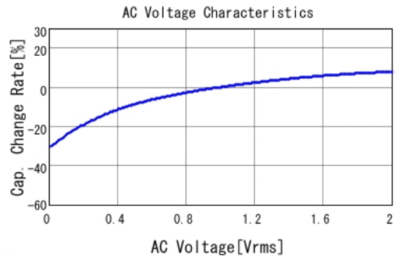
■ GRM219C71C475ME21 C-AC Voltage capchange, DCOV, 25.0d
