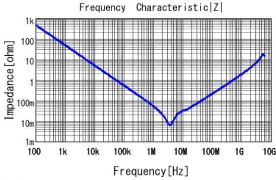
■ GRM219C81A475KE34 |Z| DCOV, 25degC
