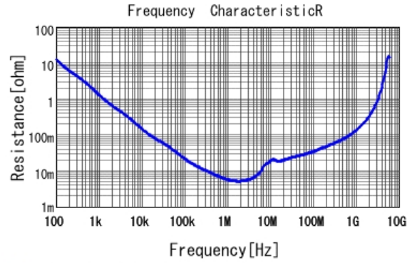
■ GRM219C81A475KE34 R DCOV, 25degC
