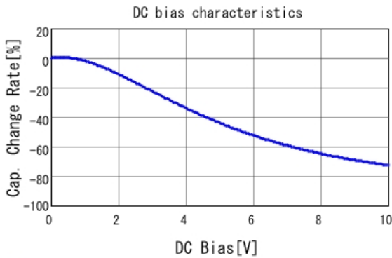
■ GRM219C81A475KE34 C-DC bias capchange, 25.0degC, AC0.
