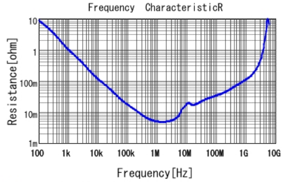
■ GRM219C81C475KA73 R DCOV, 25degC
