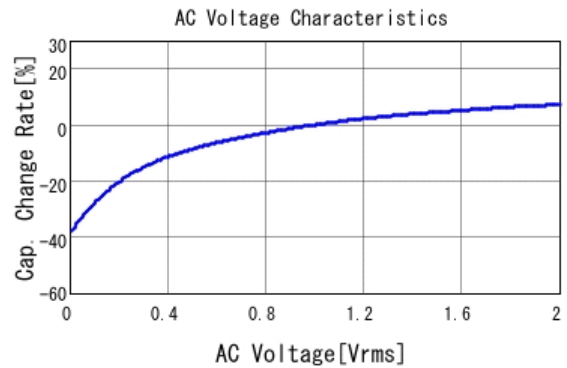
■ GRM219C81C475KA73 C-AC Voltage capchange, DCOV, 25.0d
