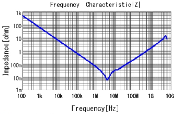
■ GRM219C81C475KA73 |Z| DCOV, 25degC
