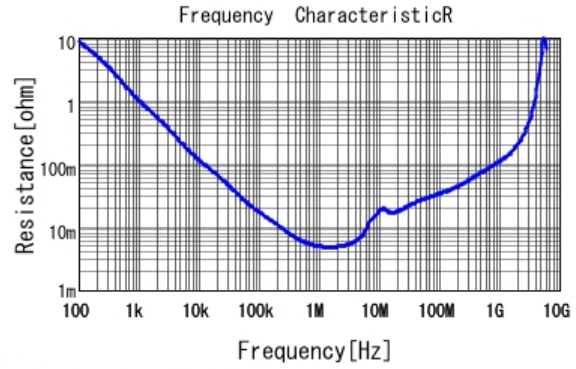
■ GRM219C81C475MA73 R DCOV, 25degC
