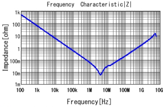
■ GRM219C81C475MA73 |Z| DCOV, 25degC
