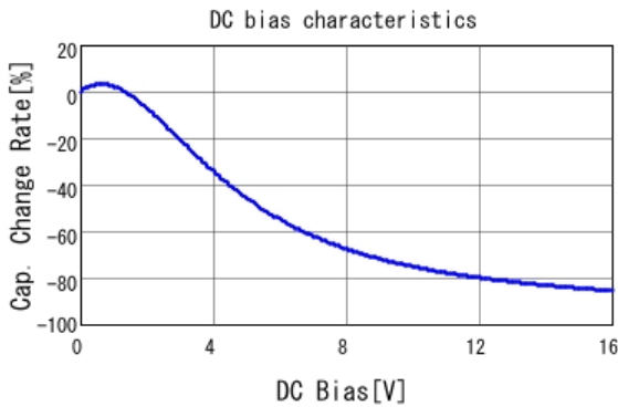
■ GRM219C81C475MA73 C-DC bias capchange, 25.0degC, AC1.
