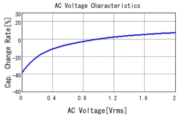
■ GRM219C81C475MA73 C-AC Voltage capchange, DCOV, 25.0d
