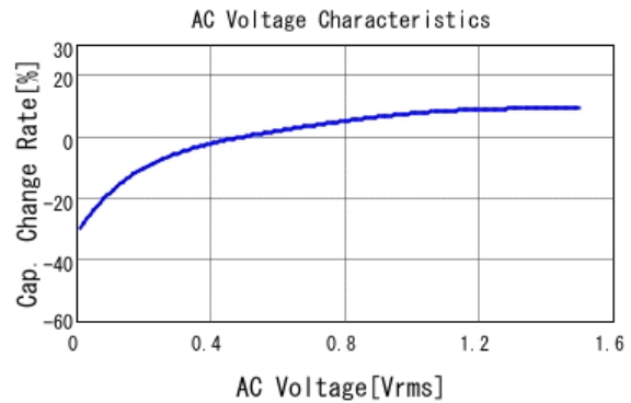
■ GRM219R60J106KE19 C-AC Voltage capchange, DCOV, 25.0d
