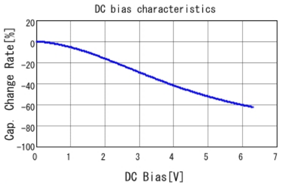
■ GRM219R60J106KE19 C-DC bias capchange, 25.0degC, AC0.
