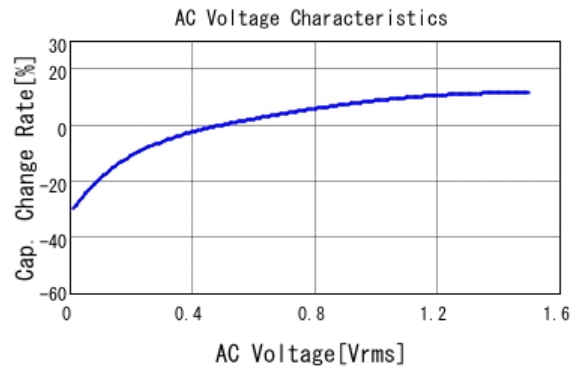
■ GRM219R61A106KE44 C-AC Voltage capchange, DCOV, 25.0d
