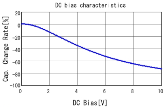
■ GRM219R61A106KE44 C-DC bias capchange, 25.0degC, AC0.
