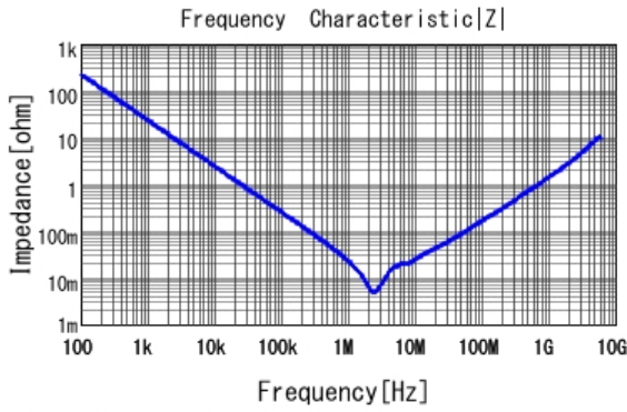
■ GRM219R61A106KE44 |Z| DCOV, 25degC
