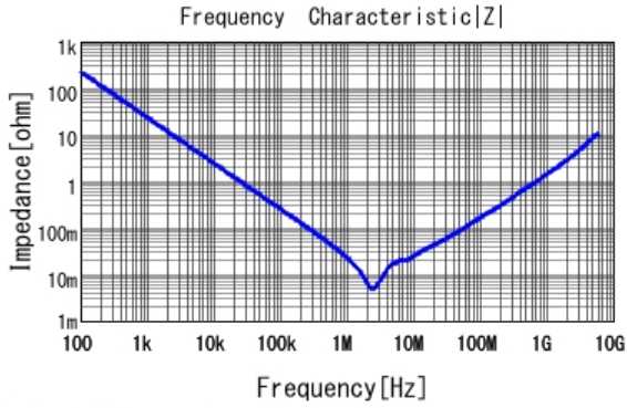
■ GRM219R61A106ME44 |Z| DCOV, 25degC
