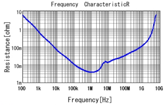
■ GRM219R61A106ME44 R DCOV, 25degC
