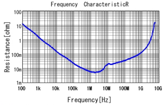
■ GRM219R61A475KE34 R DCOV, 25degC
