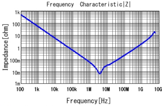
■ GRM219R61A475KE34 |Z| DCOV, 25degC
