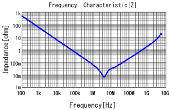
■ GRM219R61C475KE15 |Z| DCOV, 25degC
