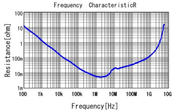
■ GRM219R61C475KE15 R DCOV, 25degC
