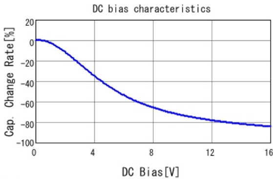
■ GRM219R61C475KE15 C-DC bias capchange, 25.0degC, AC0.
