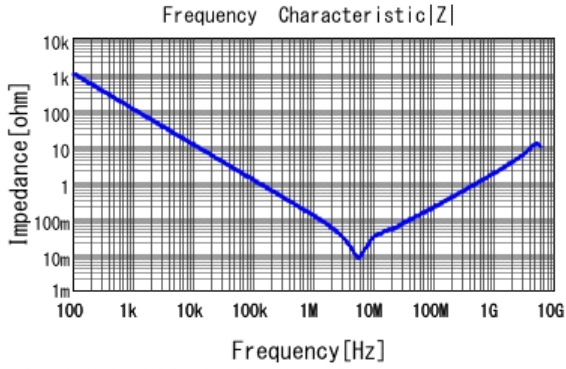
■ GRM219R61E225KA12 |Z| DCOV, 25degC
