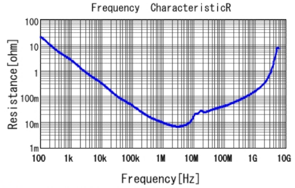
■ GRM219R61E225KA12 R DCOV, 25degC
