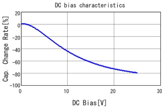
■ GRM219R61E225KA12 C-DC bias capchange, 25.0degC, AC1.
