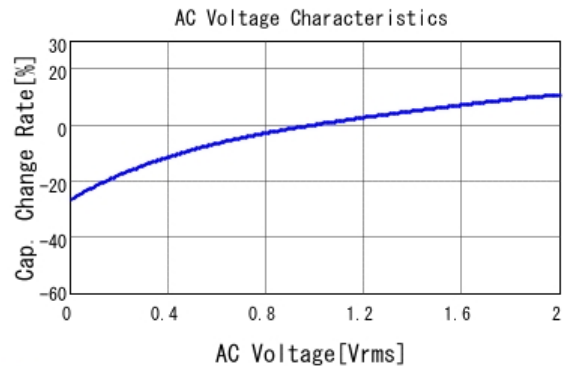
■ GRM219R61H105KA73 C-AC Voltage capchange, DCOV, 25.0d
