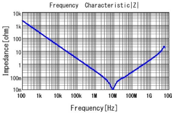
■ GRM219R61H105KA73 |Z| DCOV, 25degC
