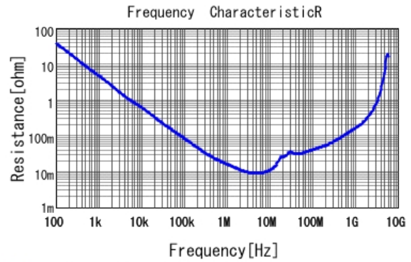
■ GRM219R61H105KA73 R DCOV, 25degC
