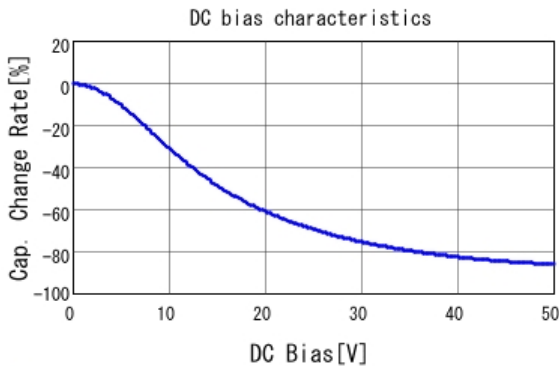
■ GRM219R61H105KA73 C-DC bias capchange, 25.0degC, AC1.
