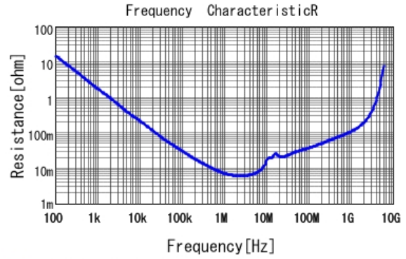
■ GRM219R61H225KE15 R DCOV, 25degC
