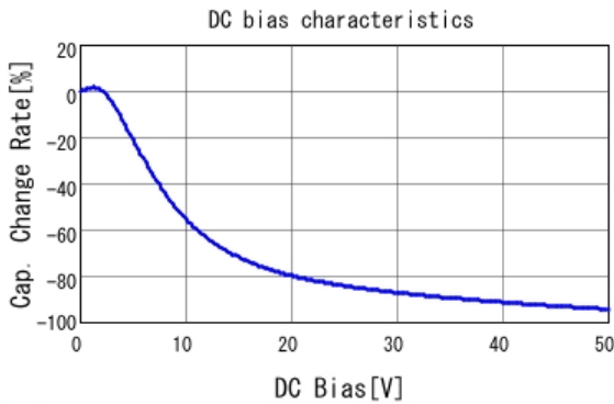
■ GRM219R61H225KE15 C-DC bias capchange, 25.0degC, AC1.
