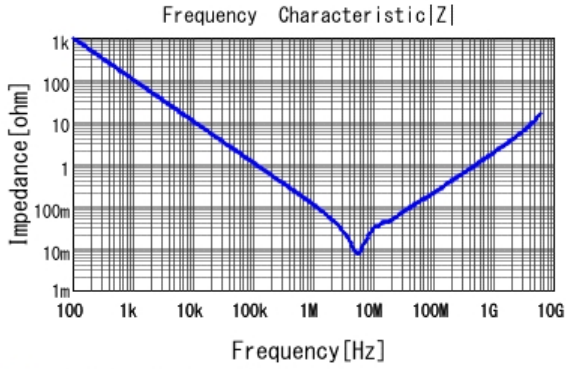
■ GRM219R61H225KE15 |Z| DCOV, 25degC
