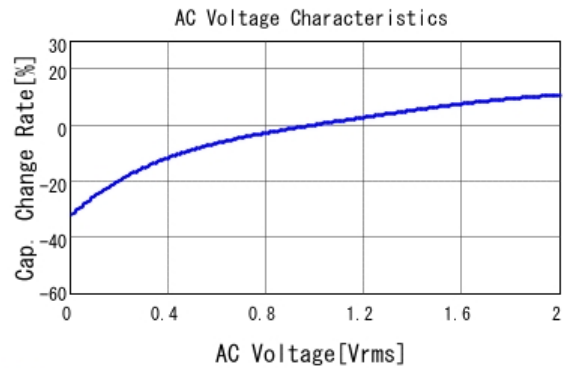
■ GRM219R61H225KE15 C-AC Voltage capchange, DCOV, 25.0d
