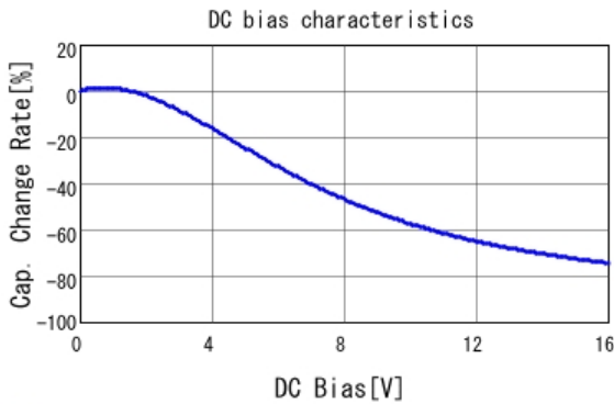
■ GRM219R71C225KE15 C-DC bias capchange, 25.0degC, AC1V
