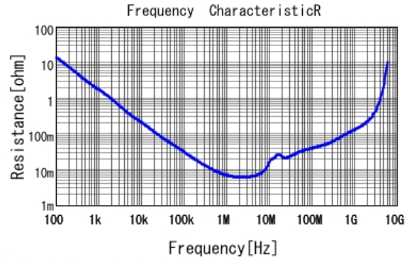
■ GRM219R71C225KE15 R DCOV, 25degC
