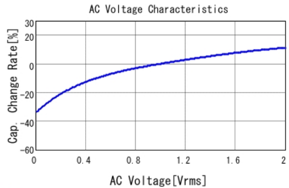
■ GRM219R71C225KE15 C-AC Voltage capchange, DCOV, 25.0d
