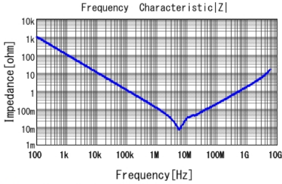
■ GRM219R71C225KE15 |Z| DCOV, 25degC
