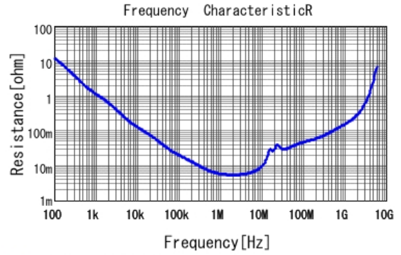
■ GRM219R71C684KA01 R DCOV, 25degC
