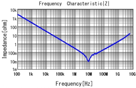
■ GRM219R71C684KA01 |Z| DCOV, 25degC
