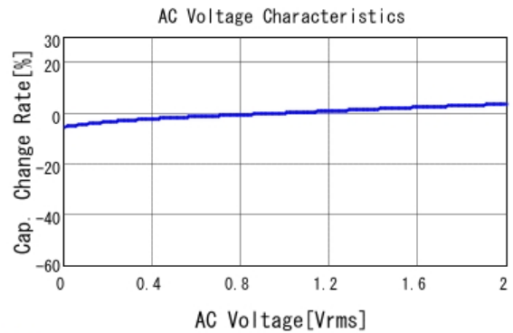
■ GRM219R71C684KA01 C-AC Voltage capchange, DCOV, 25.0d
