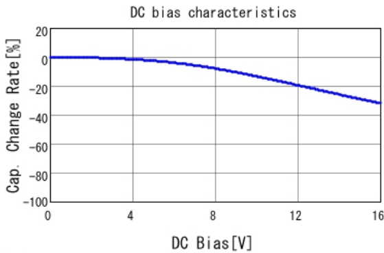
■ GRM219R71C684KA01 C-DC bias capchange, 25.0degC, AC1.
