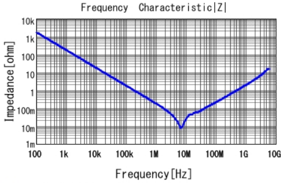
■ GRM219R71E105KA88 |Z| DCOV, 25degC
