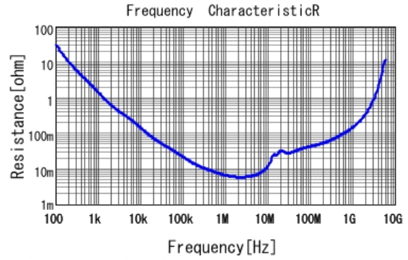
■ GRM219R71E105KA88 R DCOV, 25degC
