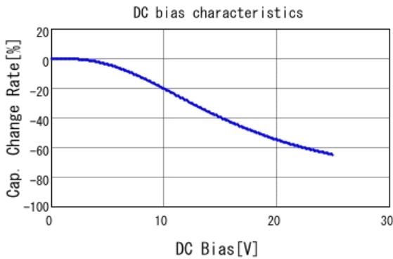
■ GRM219R71E105KA88 C-DC bias capchange, 25.0degC, AC1.
