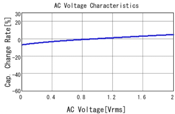
■ GRM219R71E105KA88 C-AC Voltage capchange, DCOV, 25.0d
