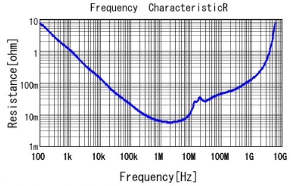
■ GRM219R7YA105KA12 R DCOV, 25degC
