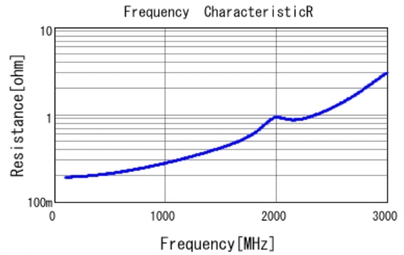
■ GRM21A5C2E680JW01 R DC0V, 25degC
