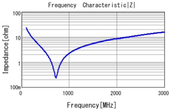
■ GRM21A5C2E680JW01 |Z| DC0V, 25degC
