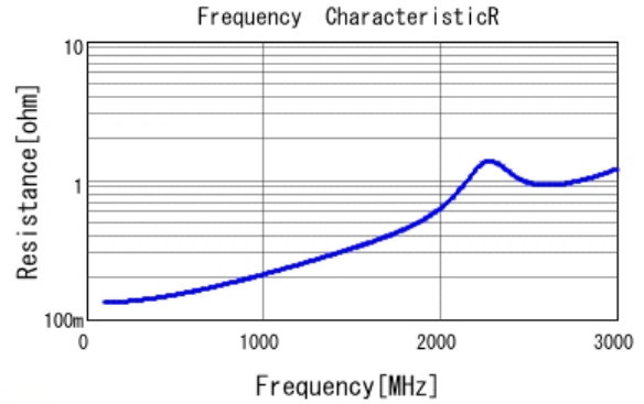
■ GRM21A5C2J680JWA1 R DCOV, 25degC
