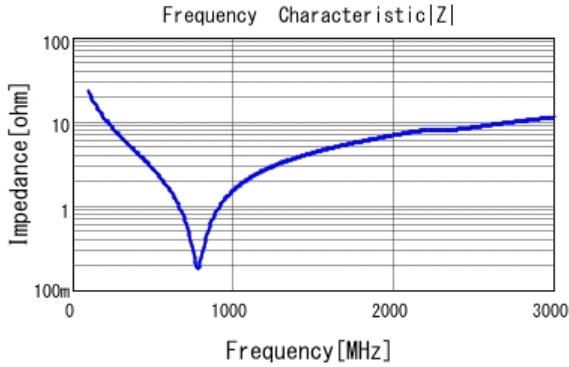
■ GRM21A5C2J680JWA1 |Z| DCOV, 25degC
