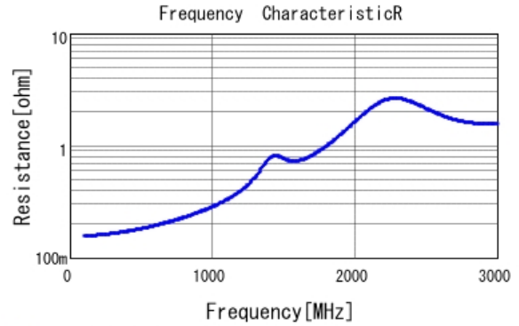
■ GRM21A7U2E101JW31 R DC0V, 25degC
