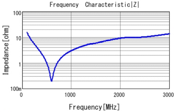
■ GRM21A7U2E101JW31 |Z| DC0V, 25degC
