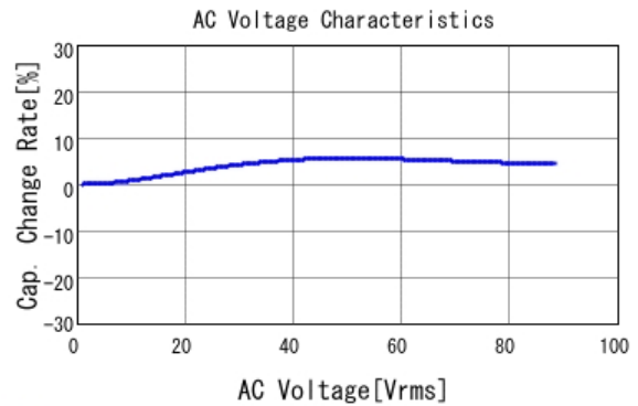
■ GRM21A7U2E221JW31 C-AC Voltage capchange, DCOV, 25.0d
