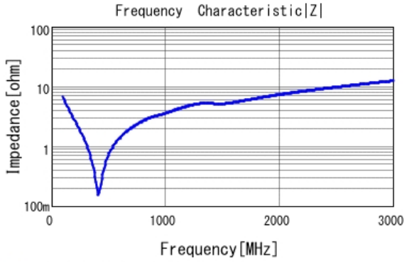
■ GRM21A7U2E221JW31 |Z| DCOV, 25degC
