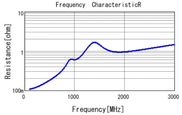
■ GRM21A7U2E221JW31 R DCOV, 25degC
