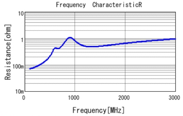
■ GRM21A7U2E471JW31 R DCOV, 25degC
