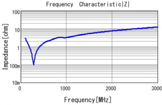
■ GRM21A7U2E471JW31 |Z| DCOV, 25degC
