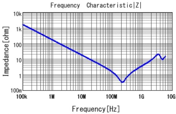
■ GRM21AR72E102KW01 |Z| DCOV, 25degC
