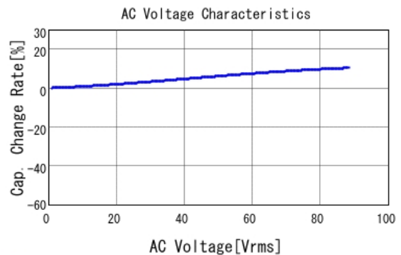
■ GRM21AR72E102KW01 C-AC Voltage capchange, DCOV, 25.0d
