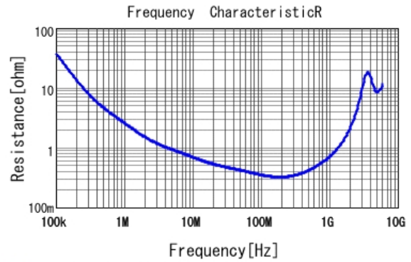
■ GRM21AR72E102KW01 R DCOV, 25degC
