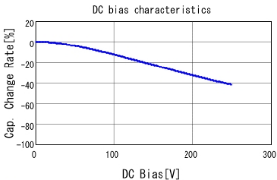
■ GRM21AR72E102KW01 C-DC bias capchange, 25.0degC, AC1V
