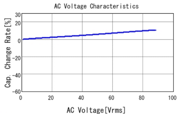
■ GRM21AR72E152KW01 C-AC Voltage capchange, DCOV, 25.0d
