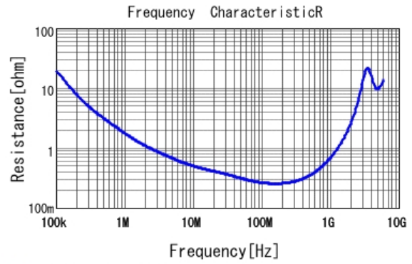
■ GRM21AR72E152KW01 R DCOV, 25degC
