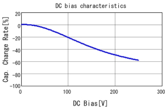
■ GRM21AR72E152KW01 C-DC bias capchange, 25.0degC, AC1V
