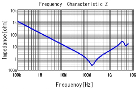
■ GRM21AR72E152KW01 |Z| DCOV, 25degC
