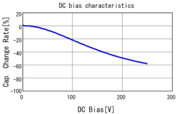
■ GRM21AR72E222KW01 C-DC bias capchange, 25.0degC, AC1V
