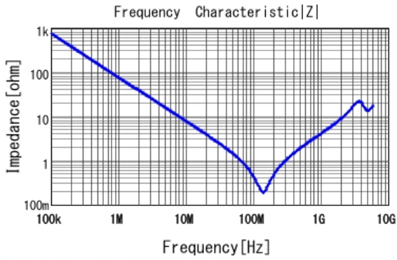
■ GRM21AR72E222KW01 |Z| DCOV, 25degC
