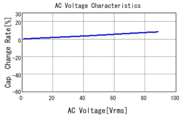
■ GRM21AR72E222KW01 C-AC Voltage capchange, DCOV, 25.0d
