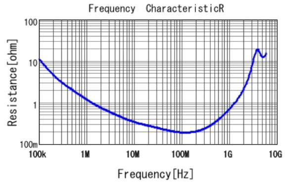
■ GRM21AR72E222KW01 R DCOV, 25degC
